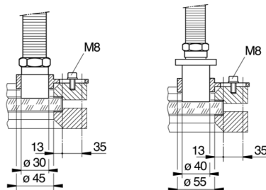
Lightpipe:
